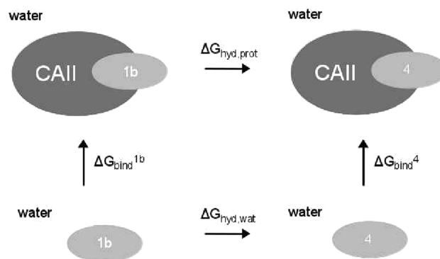
Figure 7. Free energy cycle used to calculate the difference in binding free energy between compound 4 and 1b ( \Delta\Delta G_{\text{bind}} = \Delta G_{\text{bind}}^4 - \Delta G_{\text{bind}}^{1b} = \Delta G_{\text{hyd,prot}} - \Delta G_{\text{hyd,wat}} ).
