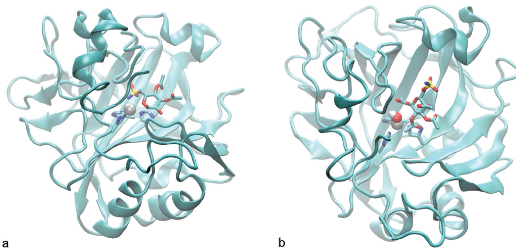
Figure 6. Active site structure of hCA II with the ligand inside the pocket. (a) Pure inhibitor conformation of compound 4 (X-ray structure CA II:1b_4) and (b) substrate conformation of the parent sulfamate 1b (docking structure). Highlighted are the zinc (gray sphere), hydroxide (red-white spheres), ligand (licorice), and histidine residues (licorice in the background).
