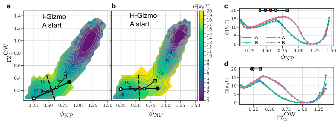
FIGURE 5 2D (a and b) and 1D (c and d) PMFs of pore nucleation for headgroup and water CVs, \phi_{NP} and rz_4^{OW} . The formatting is as in Fig. 4. The \mathcal{T} overlays in (c) and (d) are from the H-gizmo committor ensemble. To see this figure in color, go online.
